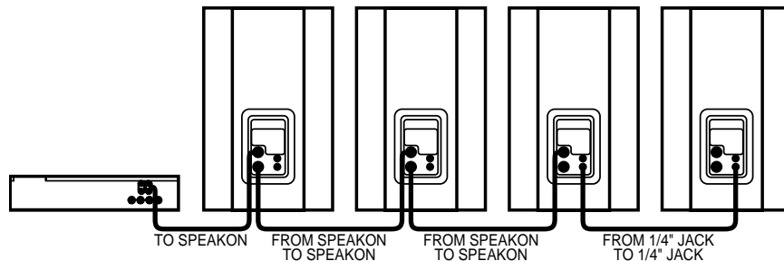
Figure 1: Multiple Speaker Interconnection Diagram
